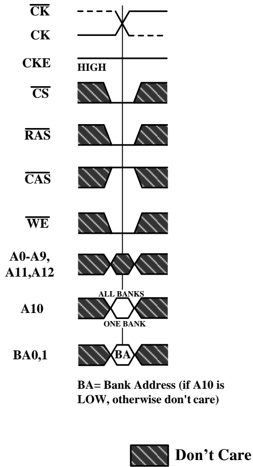
Figure 28. Precharge Command
