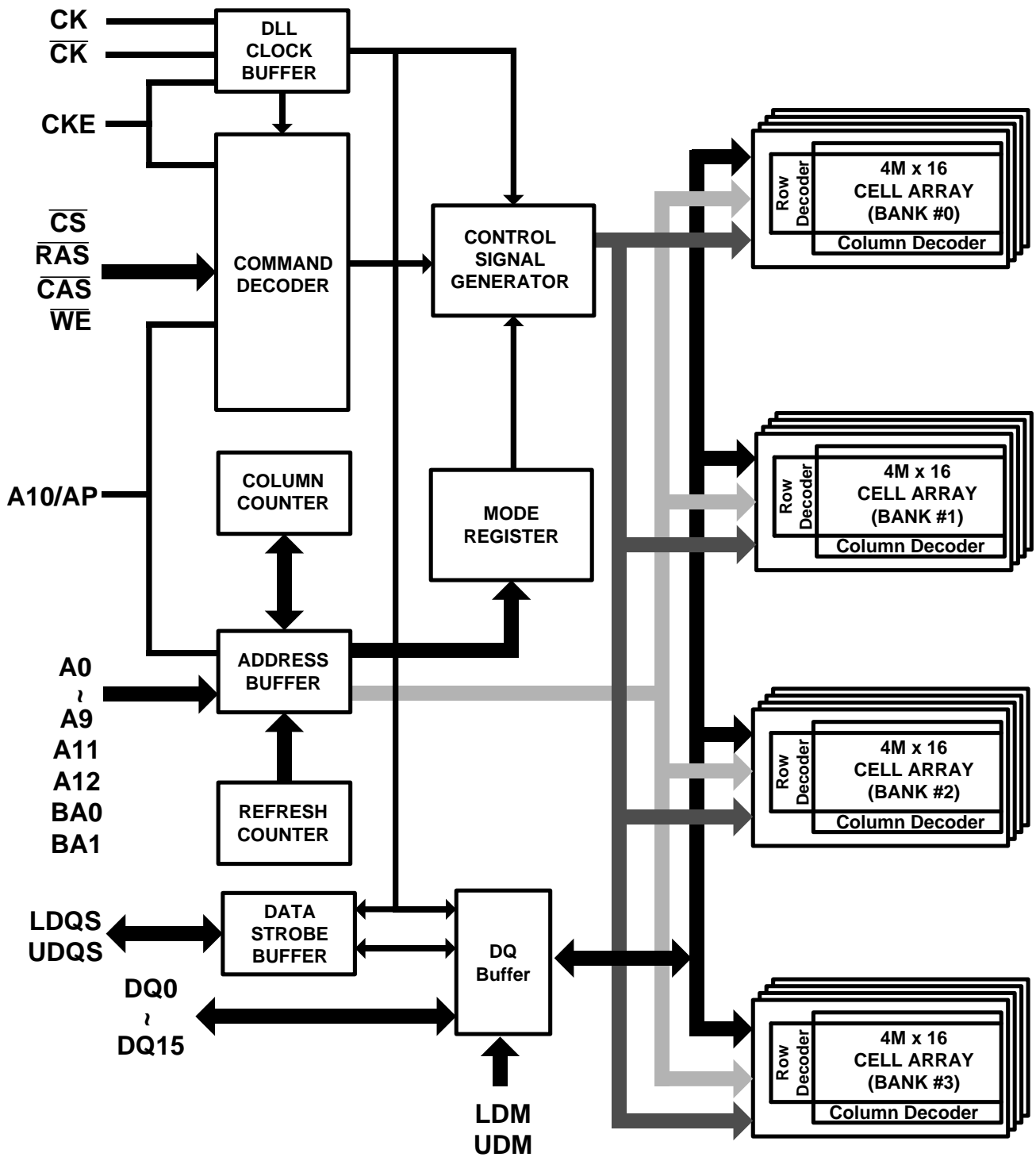
Figure 3. Block Diagram
