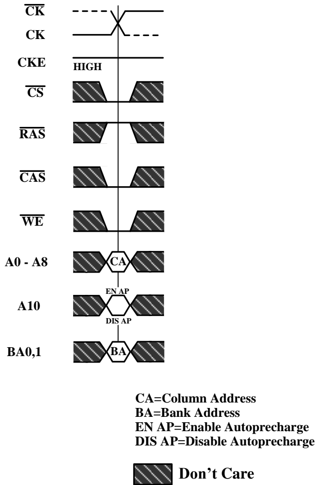
Figure 15. Write Command
