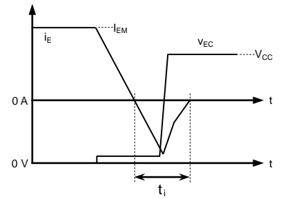
Turn-on / Turn-off switching energy and Reverse recovery energy test waveforms (Integral time t_i instruction drawing)
