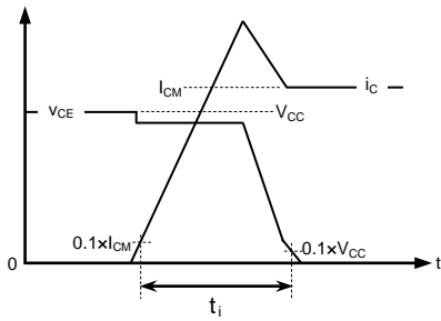
Turn-on / Turn-off switching energy and Reverse recovery energy test waveforms (Integral time t_i instruction drawing)
