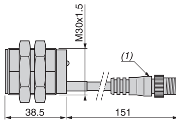
(1) M12 4-pin connector.
